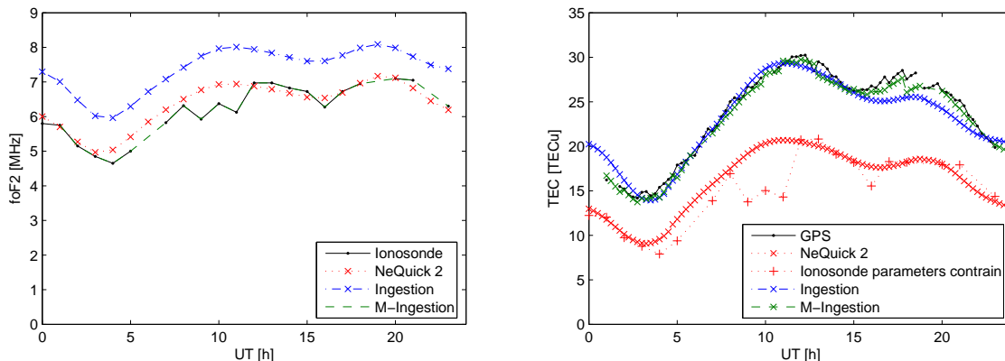
Figure 1: foF2 (left) and vTEC (right) comparison for different uses of NeQuick 2 (Dourbes, July 26 th , 2002)
