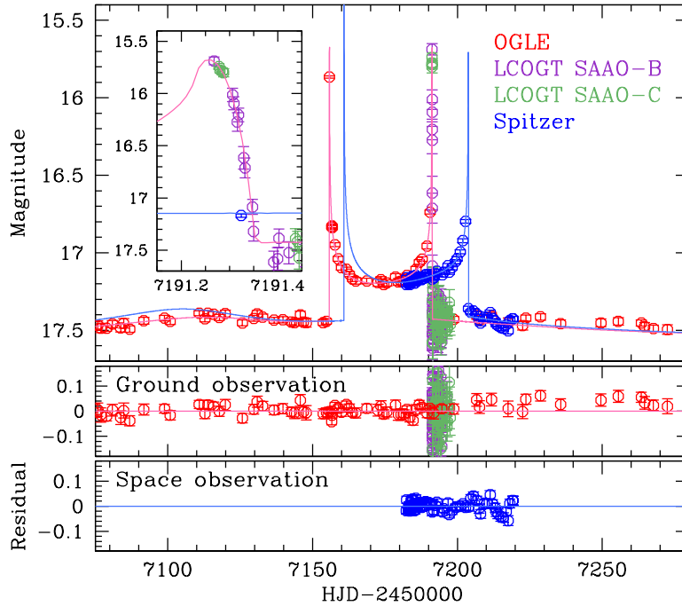
FIG. 1.— Light curves of the microlensing event OGLE-2015-BLG-0479 as seen from the Earth and from the Spitzer telescope. Superposed on the data points are the best-fit model curves obtained considering space-based parallax effects. The inset shows an enlargement of the caustic-exit part of the light curve seen from Earth. The two lower panels show the residuals from the model for the ground-based and space-based data sets.
