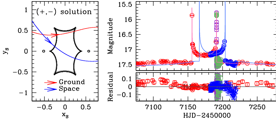
FIG. 3.— The lens system geometry and the light curve corresponding to the (+, -) local solution. Notations are same as those in Fig. 1 and 2.
