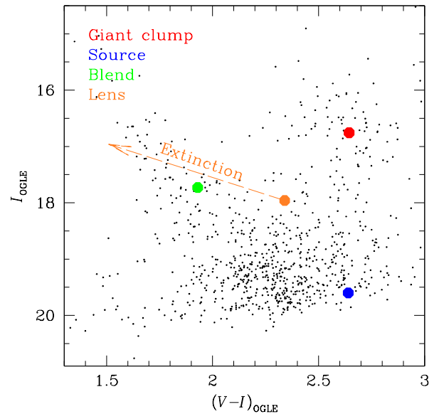
FIG. 4.— Position of the source star with respect to the centroid of giant clump in the instrumental color-magnitude diagram. Also presented are the positions of the blend and the lens. The lens position is estimated under the assumption that the lens and clump giants experience the same amount of reddening and extinction. The arrow starting from the lens position represents one magnitude difference in extinction (relative to the clump), under the assumption that the ratio of total-to-selective extinction is R_{VI} = A_I/E(V-I) = 1.31 . Hence, if the blend is the lens, then the lens is less extinguished by \Delta A_I \simeq 0.5 .
