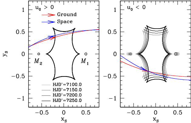
FIG. 2.— Geometry of the lens system for the u_0 > 0 (left panel) and u_0 < 0 (right panel) solutions. In each panel, the closed curve with 6 cusps represents the caustic formed by the binary lens. The locations of the binary lens components ( M_1 and M_2 < M_1 ) are marked by small open circles. The red and blue curves with arrows are the source trajectories as seen from Earth and from the Spitzer telescope, respectively. We note that the positions of the lens components and the shape of the caustic vary in time due to the orbital motion of the binary lens. We present the positions of the lens and caustic at 4 different times marked in the legend. We note that the variation of the caustic for the u_0 > 0 model is very small due to the small value of the orbital parameter ds_{\perp}/dt and thus 4 different caustics appear to be a single caustic. All lengths are normalized to the angular Einstein radius corresponding to the total mass of the binary lens.
