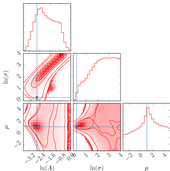
Fig. 1. Probability density functions for the three parameters used in the log-normal fit described in the text: \ln(A) , \ln(\sigma) , and \mu (red histograms). Also shown are the correlations between parameters where reds are highest and whites are lowest values of the likelihoods. Also noted in blue are the locations of the parameter values in the MLE fit described in the text.
