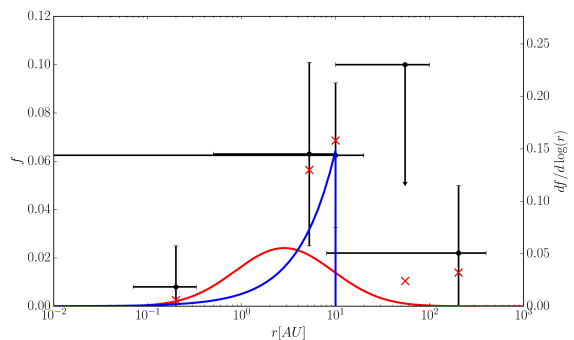
Fig. 2. Log-normal surface density distribution of 1–10 M_J Companions to M dwarfs. On the left axis are the integrated values of f , where the black points correspond to the data points listed in Table 1: note the horizontal lines are ranges while the vertical lines are errors in f . On the right axis are the relative values of the differential PDFs. In red is the MLE fit as described in the text. The integrated f values for the MLE, over the ranges in semi-major axis corresponding to the data from Table 1, are shown as red “x”. Also shown in blue is the fit from Clanton & Gaudi (2016) which was published before the Lannier et al. (2016) results were available.
