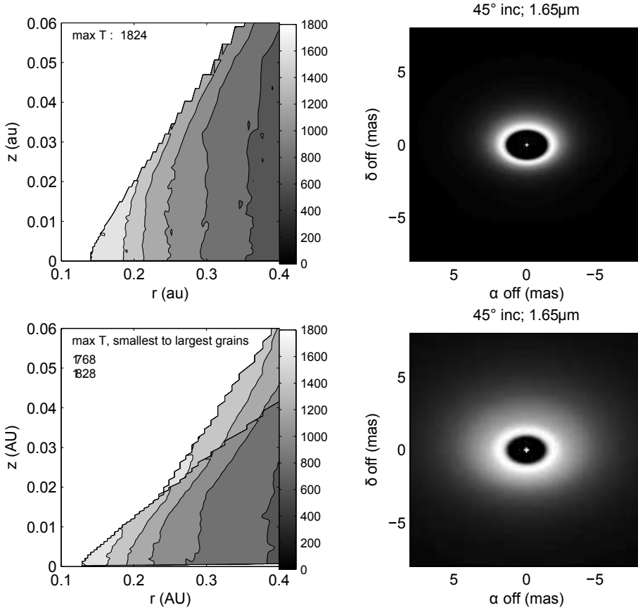
Fig. 11. Graphical summary of models IN (above) and THM (below). Left: temperature profiles; in the case of the THM model, the temperature distributions for large grains is overlaid onto that for small grains. Right: sky images at \lambda = 1.65 \mu\text{m} , i = 45^\circ ; a mild enhancement of low brightness regions has been realized by a square root scaling. The angular scale is for the object located at a distance of 100 parsecs.
