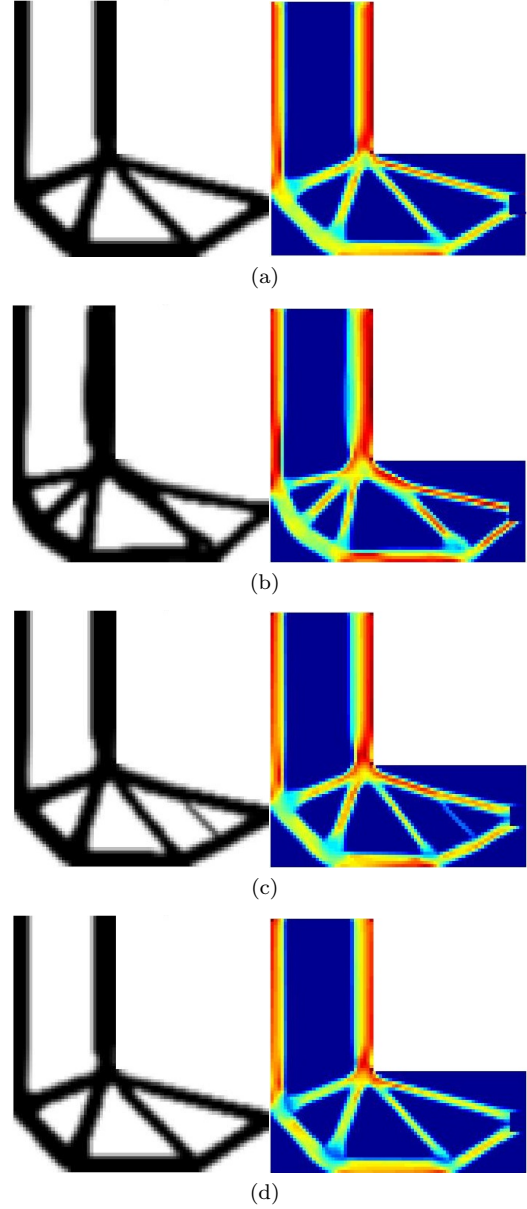
Fig. 7 Example 2. Optimized topologies and relevant stress maps for the MWCS and MWCF formulations of Example 2: (a) MWCS, (b) MWCF 1 ( c_a = 0.7; c_m = 0.3 ), (c) MWCF 2 ( c_a = 0.5; c_m = 0.5 ) and (d) MWCF 3 ( c_a = 0.3; c_m = 0.7 )
