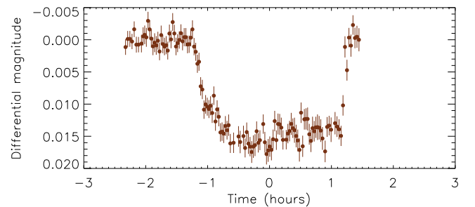
Figure 3. The CASLEO light curve of WASP-103. Times are given relative to the mid-point of the transit.
