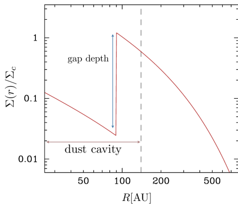
FIG. 7.— Model surface density profile (Equation 6) of the disk.
