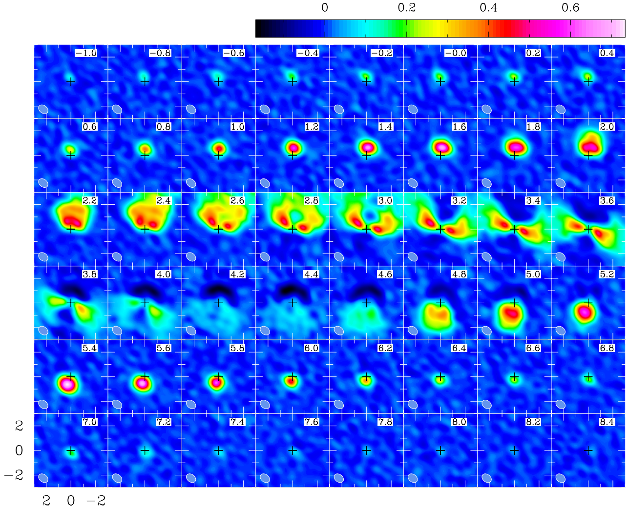
FIG. 3.— ^{12}\text{CO } J = 2 - 1 channel maps from CLEAN reconstruction in an exponential color scale. The LSR velocity for each channel is indicated in the upper right-hand corner in \text{km s}^{-1} . North is up, East is to the left. The systemic velocity of HD 142527 is 3.6 \text{ km s}^{-1} . The synthesized beam is shown in the lower left-hand corner. The cross at origin represents the stellar position which most likely represents the center of rotation of the disk velocity profile. The color wedge is in units of \text{Jy beam}^{-1} \text{ km s}^{-1} . The position of the disk center, which we assume is given by the center of symmetry of the emission at systemic velocity (channel at +3.6 \text{ km s}^{-1} ), is consistent with the estimated astrometry after correcting by the source's proper motion (black cross).
