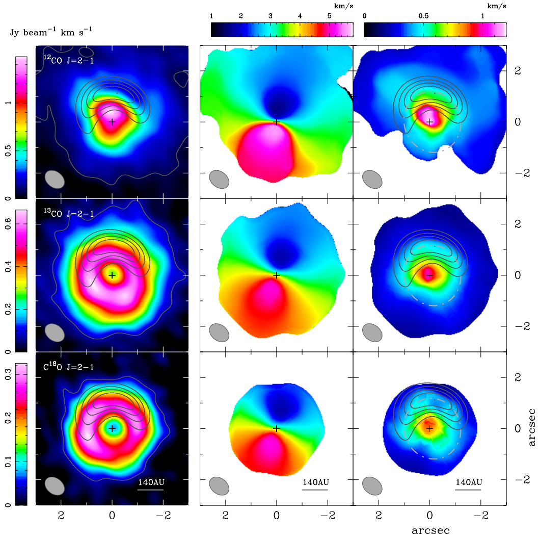
FIG. 1.— Moment maps carbon monoxide isotopologues ^{12}\text{CO} , ^{13}\text{CO} and \text{C}^{18}\text{O} J = 2 - 1 . North is up, East is left. Left : Moment zero; continuum subtracted integrated line emission, considering flux contribution from all channels from -0.8 to +7.8 \text{km s}^{-1} , in units of \text{Jy beam}^{-1} \text{km s}^{-1} . Continuum at 230 GHz is shown in contours. The ^{12}\text{CO} map shows the large extent of the molecular line emission, the north-south asymmetry is due to foreground absorption. ^{13}\text{CO} and \text{C}^{18}\text{O} show a central cavity. The noise level for all intensity maps is about 1\sigma = 11 mJy per beam. Center : First moment showing the velocity map. The coordinates origin is set to the center of the disk and it is marked with a cross. The synthesized beam is shown in the lower left corner. The dashed ellipse in the moment 2 map is a fit by inspection of the dust-continuum horseshoe border. The ellipse shows that there is a difference in dispersion of the gas under the horseshoe, with respect to the south counterpart of the disk.
