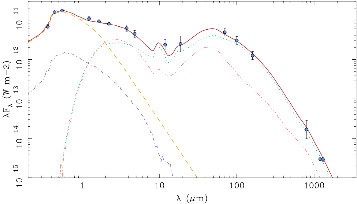
FIG. 10.— Dereddened photometry (blue dots) and spectral energy distribution model of HD142527. Photometric data points have been obtained from Verhoeff et al. (2011). We have added the new ALMA continuum photometry at 1.2 mm. 5\sigma error bars are shown. The model contributions are: stellar spectrum alone (dashed yellow curve), scattered light from the star (dash-dotted light blue curve), thermal emission from inner and outer disks (dotted green curve), scattered light from the dust thermal emission (dash triple dotted orange curve). The resulting model is the red solid curve.
