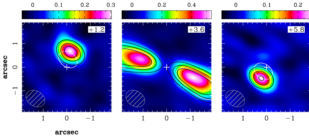
FIG. 9.— These panels show the bestfit model for the disk structure in HD 142527 in ^{13}\text{CO} emission. The model is presented in contours while the ALMA data are shown in false color. Black contours show the model with an inclination angle of 28 degrees and a central star mass of 2.2 M_{\odot} , which best reproduces the observed morphology. The white contours show a similar model but with a disk inclination of 20 degrees only. Left : Blue high velocity channel that shows gas coming from inside the cavity, close to the central. Center : Systemic velocity channel. Right : Red high velocity channel. See top wedge for contours and emission levels.
