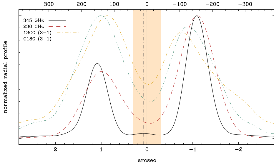
FIG. 6.— HD 142527 disk profile cuts extracted from the zeroth order moment maps (at 2h). Solid black and dashed red lines show integrated intensity of 345 GHz and 230 GHz continuum, respectively. ^{13}\text{CO} and \text{C}^{18}\text{O} J = 2 - 1 emission integrated intensity cuts are shown in yellow dot-dash and green dot-dot-dash lines. The shaded region shows the size of the beam across the cut axis. The extracted cuts have been scaled to the 345 GHz continuum peak to aid comparison between gas emission and dust. The bottom and top x -axes are in arcsec and au, respectively. The beam size at 345 GHz is 0.51'' \times 0.33'' . The x -axis origin (solid vertical line) is given by the mid point in between the two 345 GHz peaks, determined by fitting single gaussians. The vertical dot-dashed line indicates the centroid of the faint central emission (see Section 3.2).
