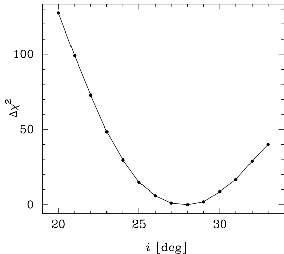
FIG. 8.— Plot of \Delta\chi^2 as a function of a single parameter, the inclination of the disk i . The curve has a minimum around i = 28 deg, with a 1\sigma error of \pm 0.5 deg.
