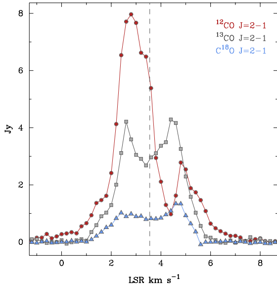
FIG. 2.— Continuum-subtracted ^{12}\text{CO} (circles), ^{13}\text{CO} (squares) and \text{C}^{18}\text{O} (triangles) J = 2 - 1 emission line spectra. The spectra are extracted by summing over the whole data cube. Vertical dotted line corresponds to systemic velocity of 3.6 \text{ km s}^{-1} , as determined from the ^{12}\text{CO} channel maps.
