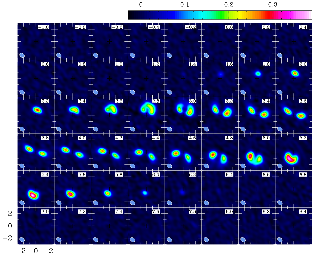
FIG. 5.— \text{C}^{18}\text{O} channel maps in linear color scale. For details, see caption in Fig. 3.
