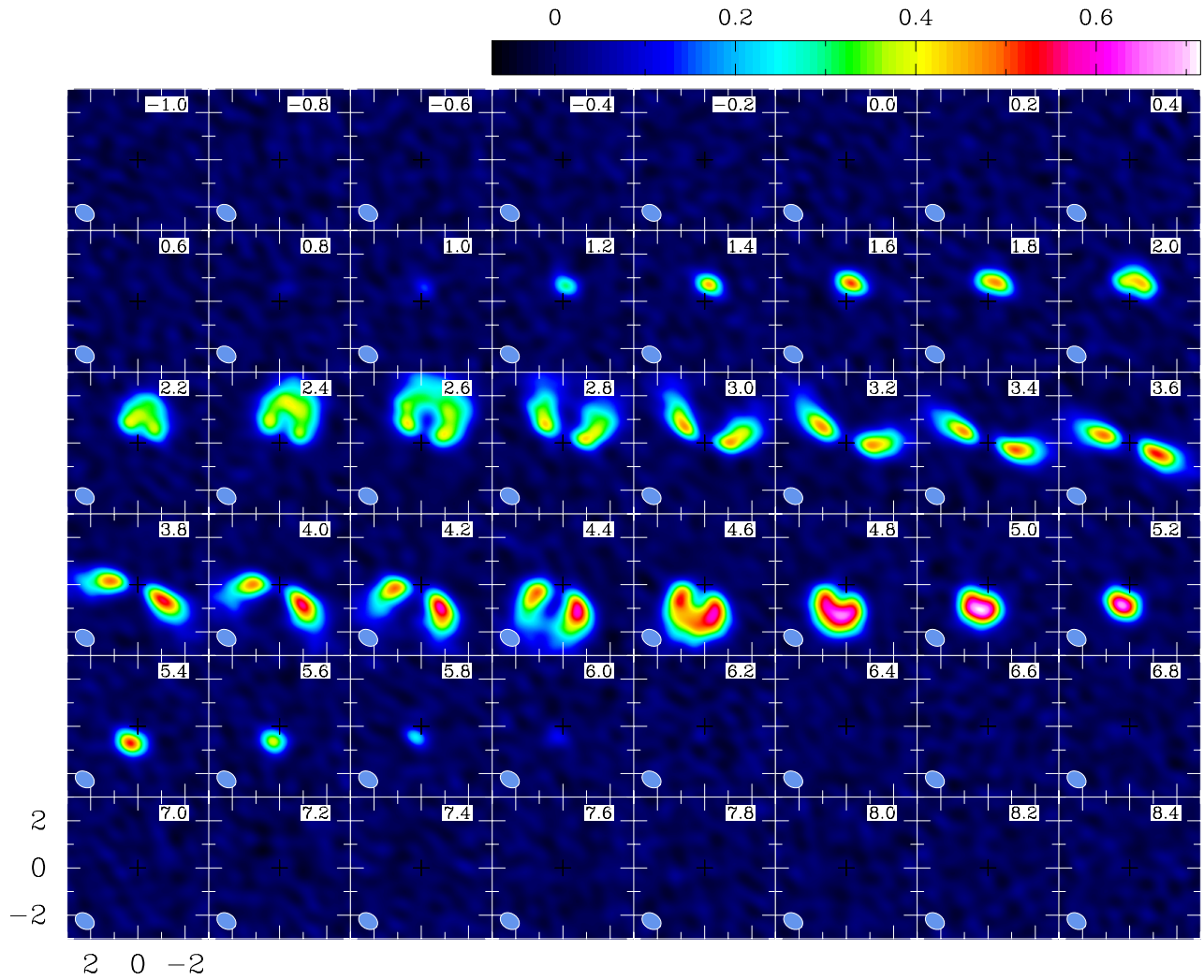
FIG. 4.— ^{13}\text{CO} channel maps in exponential color scale. For details, see caption in Fig. 3.
