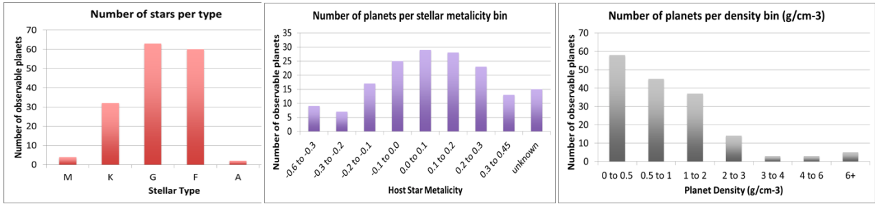
Figure 25: Known planets observable by EChO classified as function of the: Left: Stellar Type, Middle: Stellar Metallicity, Right: Planetary density in \text{g/cm}^3 .
