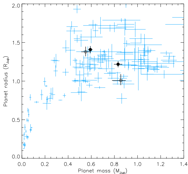
Figure 6. Plot of planet radii versus their masses. The overall population of planets is shown using blue crosses, using data taken from TEPCat on 2013 February 11. WASP-15 b and WASP-16 b are indicated using black lines with open circles for the values from their respective discovery papers and filled circles for the new results from the current work. The outlier with a mass of 0.86 M_{\text{Jup}} but with a radius of only 0.78 R_{\text{Jup}} is the recently discovered system WASP-59 (Hébrard et al. 2013).
