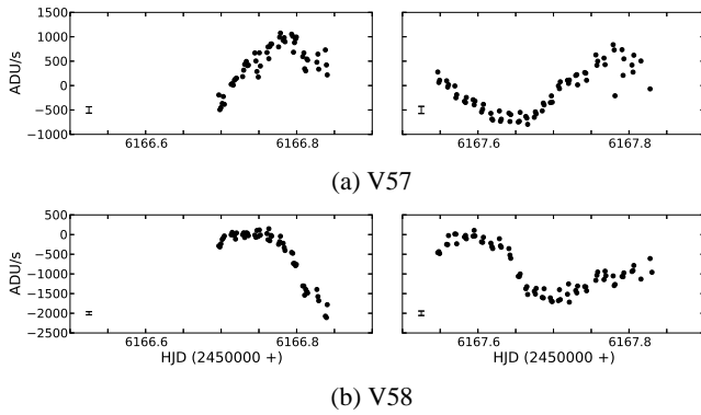
Fig. 2: Light curves, plotted in differential flux units, for the two new variable stars. Left and right panel show the first and second nights, respectively. The typical photometric uncertainty is plotted as an error bar in each panel.
