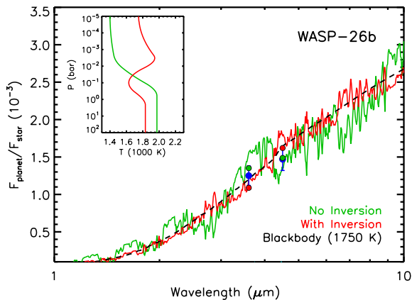
Figure 7. Spectral energy distribution of WASP-26b relative to that of its host star. The blue circles with error bars are our best-fitting occultation depths. The green line is a model-atmosphere spectrum, based on a model which assumes solar abundances in thermochemical equilibrium and lacks a temperature inversion, and the dark red line is a model with a temperature inversion. The band-integrated model fluxes are indicated with circles of the corresponding colours. The dashed black line shows a planetary black body model with a temperature of 1750K. Inset: temperature-pressure profiles for our models.
