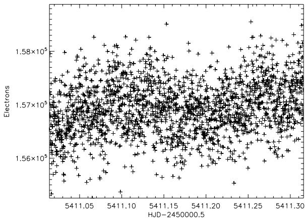
Figure 4. The raw light curve of the 4.5 \mu\text{m} Spitzer data extracted using an aperture of 2.4 pixels.
