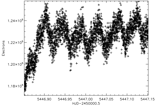
Figure 3. The raw light curve of the 3.6\mu\text{m} Spitzer data extracted using an aperture of 2.4 pixels.
