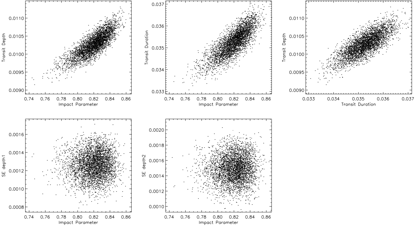
Figure 2. Correlation plots for selected proposal parameters from our MCMC analysis. For clarity we have only plotted a random 2% of the chain values.
