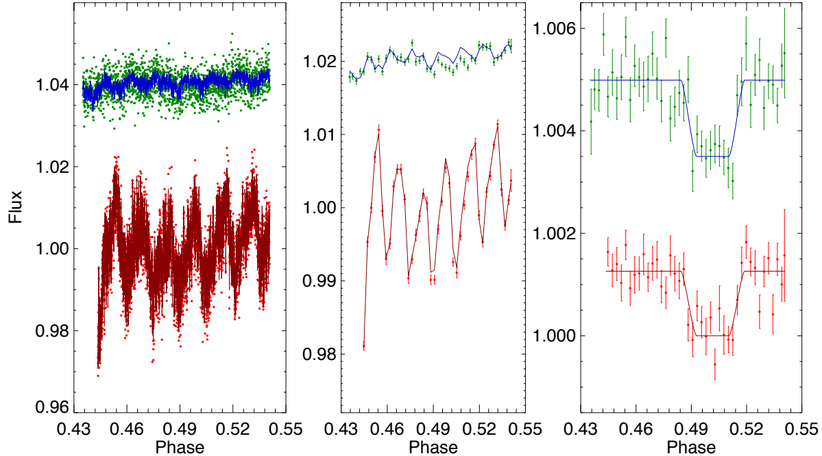
Figure 6. (Left): The raw light curves with the trend functions, the upper points are the channel 2 data and the lower points are the channel 1 data, the solid lines are the trend functions for each data set. (Middle) Binned light curves with trend models. (Right) The binned light curve with trend function removed and best fitting eclipse models (solid lines). The secondary eclipse can clearly be seen in both channels.
