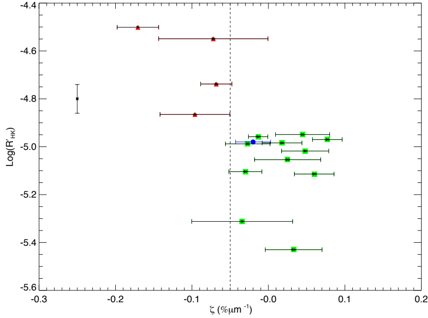
Figure 8. Activity-inversion plot for the stars in Knutson et al. (2010). Points on the left of the dotted line (triangles) are non-inverted planets around active stars and those on the right of the dotted line (squares) are inverted planets around inactive stars. The point on the left hand side of the plot shows the typical change in \log R'_{HK} (season-to-season), assuming measurements over several nights. The blue circle is WASP-26. The stars are listed in table 5.
